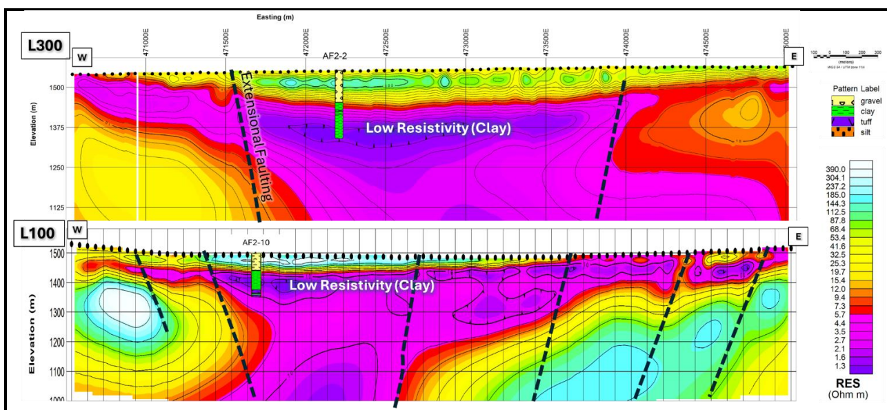
Figure 6. CSAMT 2D INVERSION DATA WITH BASIC INTERPRETATION (LINES L100 AND L300)
