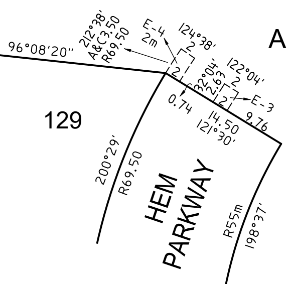
ENLARGEMENT B NOT TO SCALE
