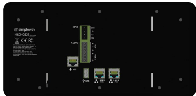
REAR VIEW
