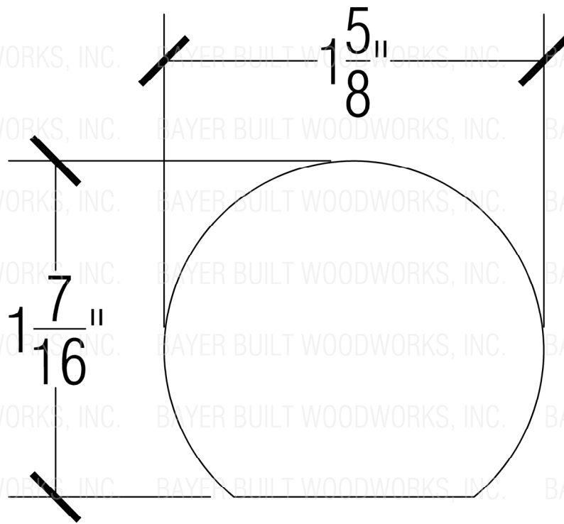
231 WALL RAIL
