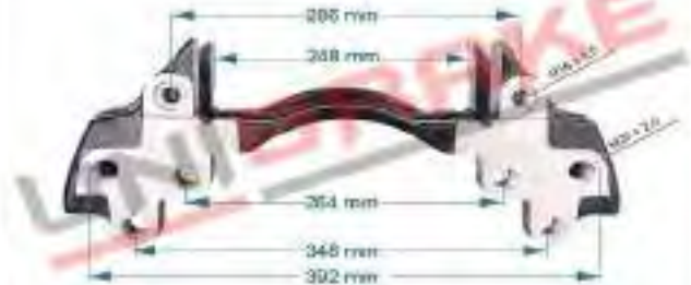
5827 / Caliper Carrier / IVECO TRUCK KNORR CARRIER KNORR: K108814K50 - K001510
