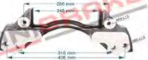
5835 / Caliper Carrier / ZF AXLE KNORR CARRIER KNORR: K001502
