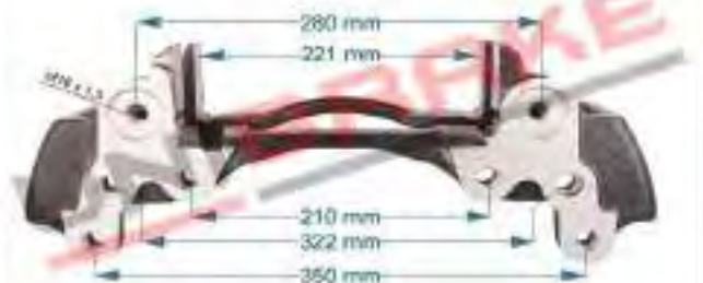
6822 / Caliper Carrier / MB AROCS REAR - LEFT WABCO CARRIER 640.915.744.4 / MB: 000 423 2306
