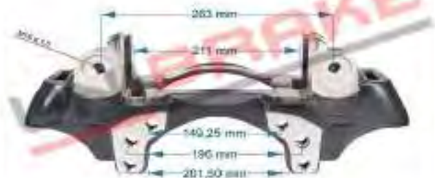
6812 / Caliper Carrier / SCHMITZ AXLE - LEFT WABCO CARRIER
