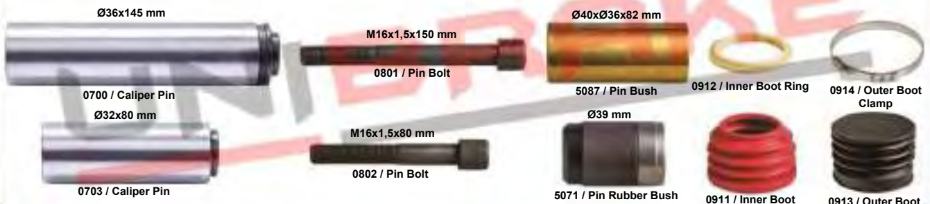
5090 / Caliper Pin Repair Kit SB6 / SB7 / SB7 Radial Type KNR: K000687 / DF: 1603326
