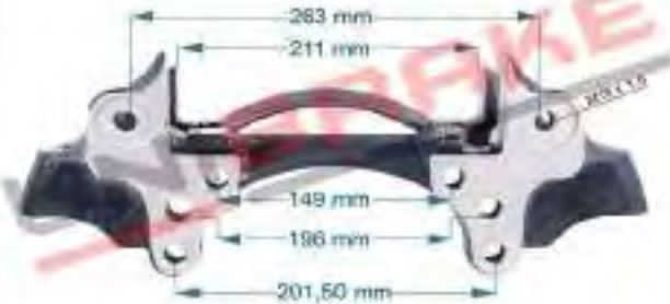
6825 / Caliper Carrier / SCHMITZ TRAILER - RIGHT WABCO CARRIER
