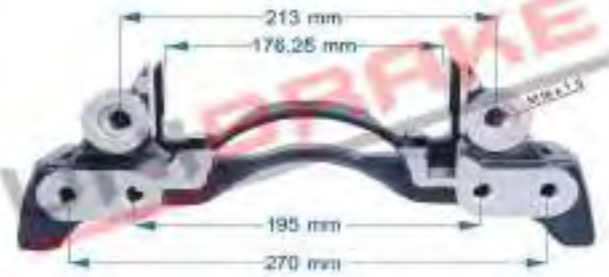
6800 / Caliper Carrier / MERCEDES FRONT - RIGHT WABCO CARRIER
