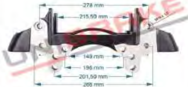
5828 / Caliper Carrier / SCHMITZ TRAILER KNORR CARRIER KNORR: K108001K50
