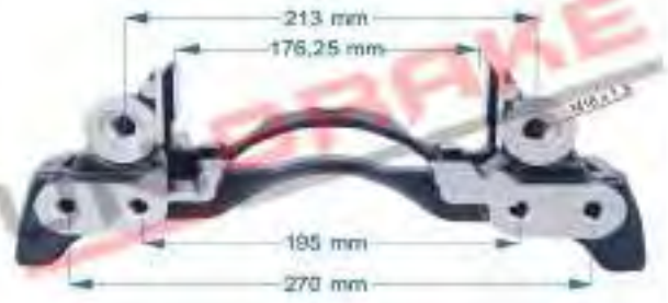
6801 / Caliper Carrier / MERCEDES FRONT - LEFT WABCO CARRIER
