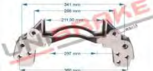
5830 / Caliper Carrier / IVECO TRUCK RIGHT KNORR CARRIER KNORR: K002314
