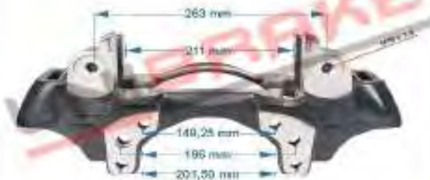
6811 / Caliper Carrier / SCHMITZ AXLE - RIGHT WABCO CARRIER
