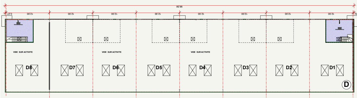
PLAN MEZZANINES
