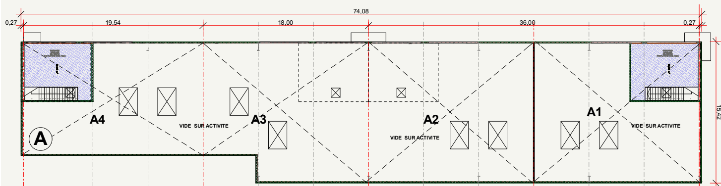
PLAN MEZZANINES
