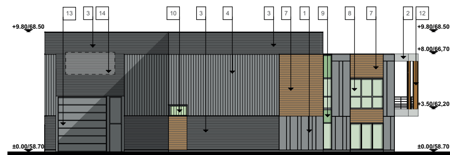
FACADE SUD
