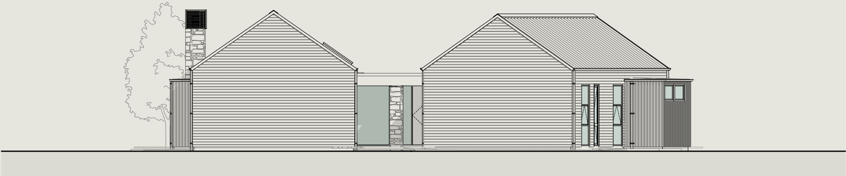
South Elevation
