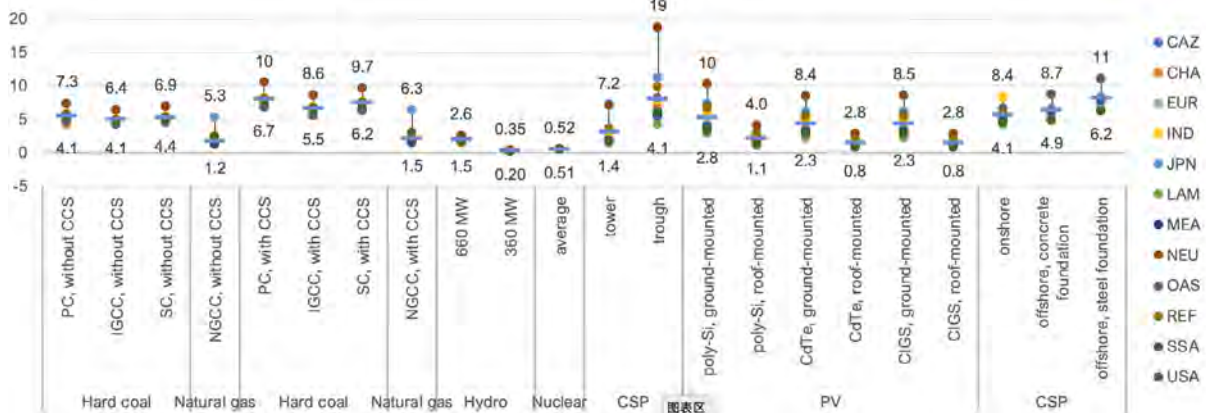
Lifecycle human toxicity potential, carcinogenic, in CTUh per TWh, regional variation, 2020
