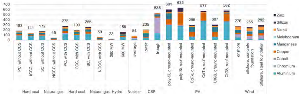
Material requirements, in g per MWh
