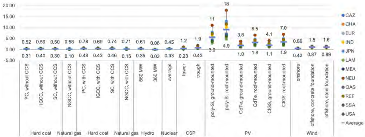
Lifecycle mineral and metal requirement, in g Sb eq. per MWh, regional variation, 2020
