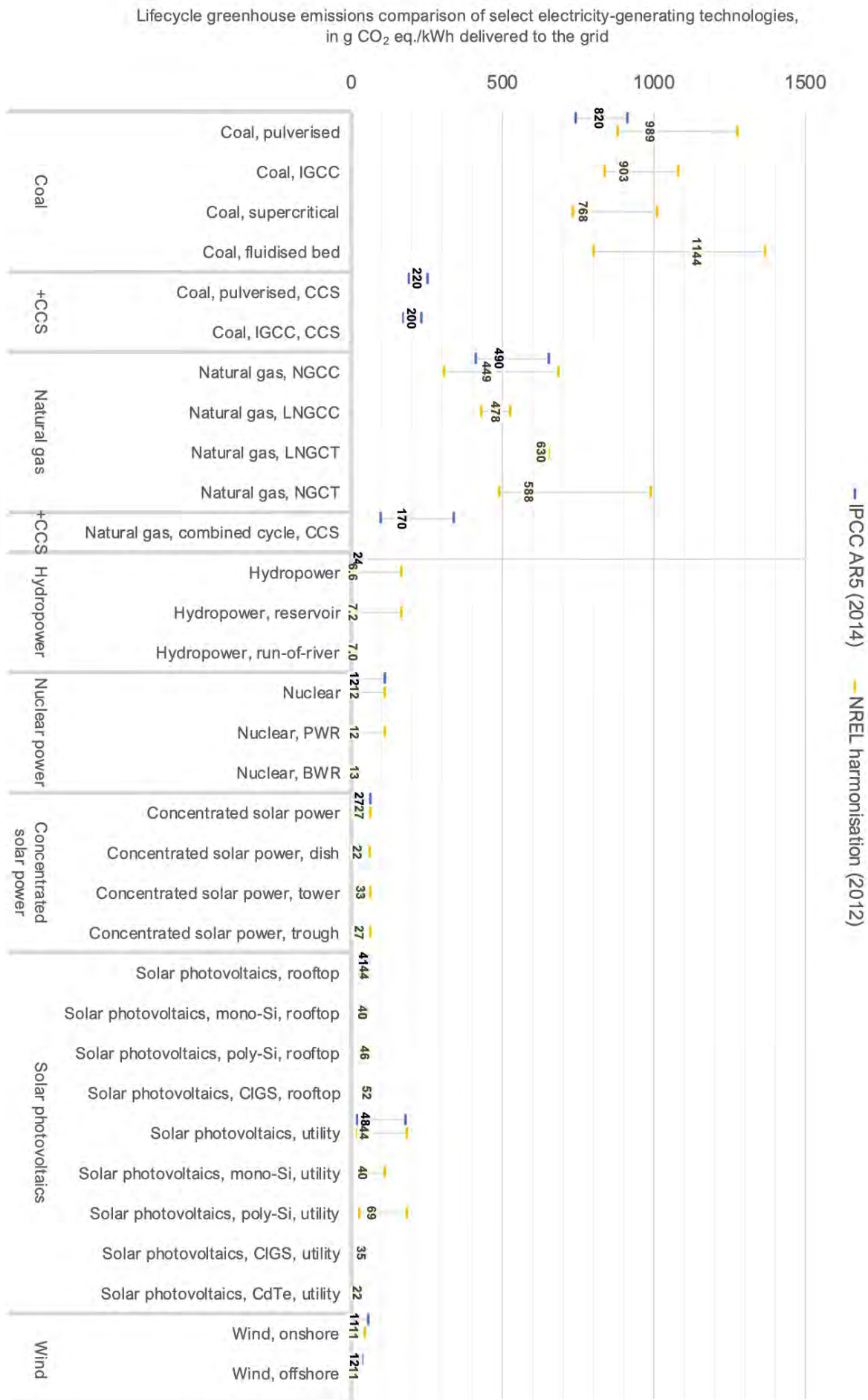
Figure 54 Lifecycle GHG emissions from electricity generation technologies, based on IPCC AR5 (2014) and the NREL harmonisation project (2012).
