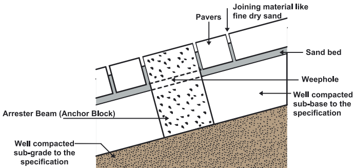
Picture shows how an Arrester Beam or Block is provided to prevent lateral movement
