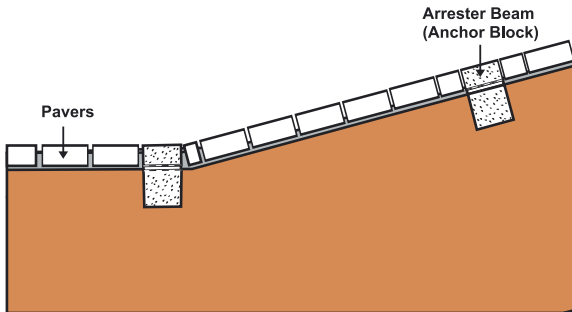
Arrester Beam (Anchor Block) can be between 25 to 60ft depending on the degree of slope
