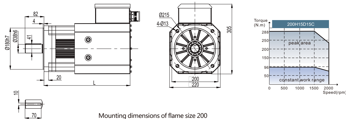
Mounting dimensions of flame size 200
