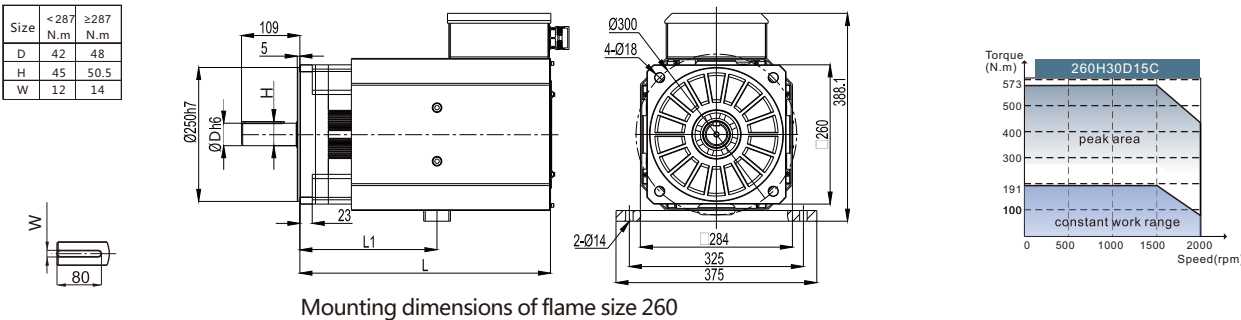
Mounting dimensions of flame size 260
