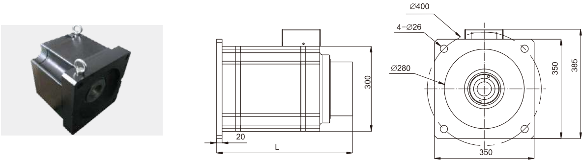
Mounting dimensions of flame size 300
