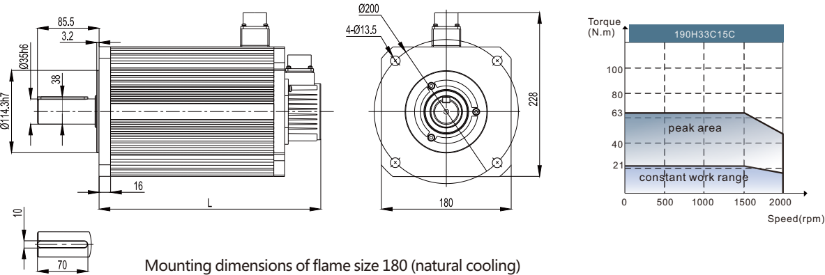
Mounting dimensions of flame size 180 (natural cooling)
