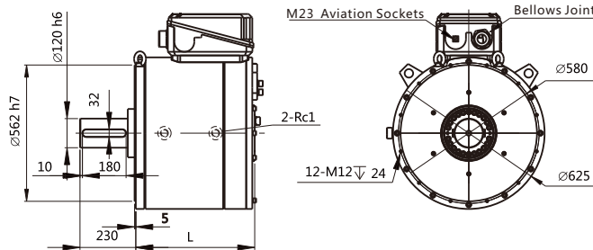
Mounting dimensions of flame size 630(Type B)
