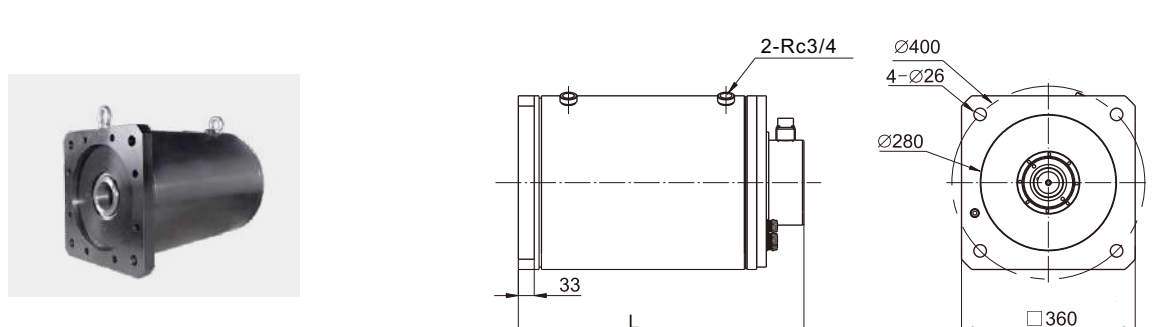
Mounting dimensions of flame size 360
