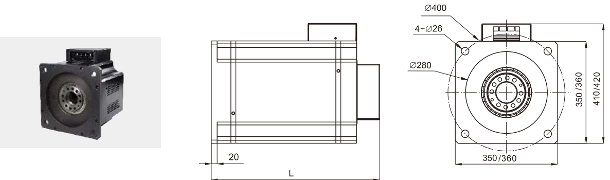
Mounting dimensions of flame size 350/360
