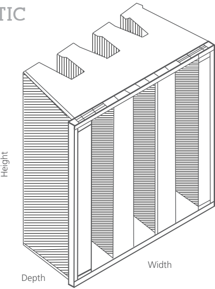
(20 mm Header) General Isometric view
