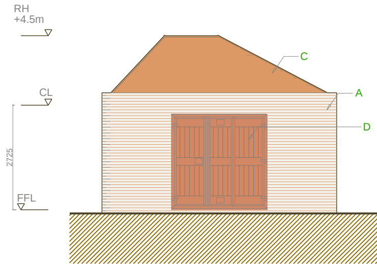
EAST ELEVATION
