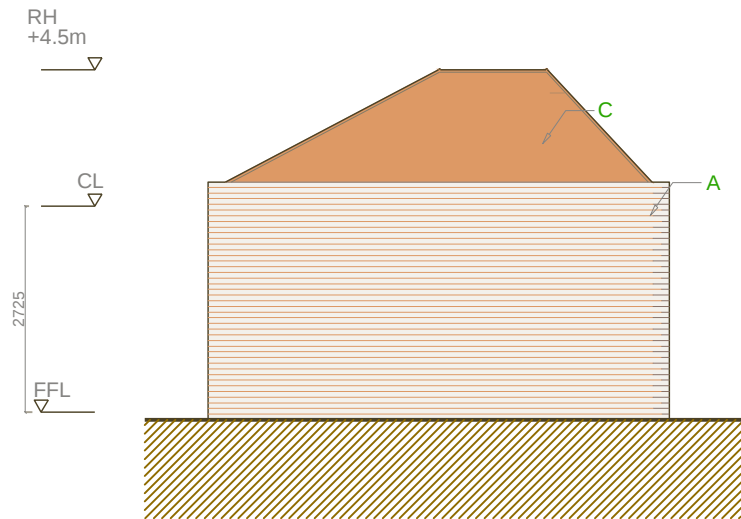
WEST ELEVATION
