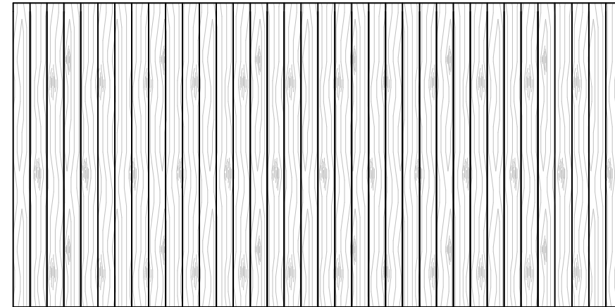
2 CedarPlank WoodCast - WALL FRONT VIEW SCALE: 3/8"= 1'-0"
