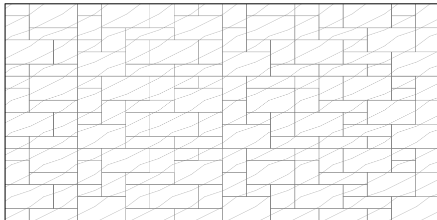
3 Ashlar Dry StoneCast - WALL FRONT VIEW SCALE: 3/8"= 1'-0"
