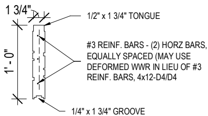
CHISELED STONE PANEL - SECTION
