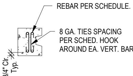
END POST
