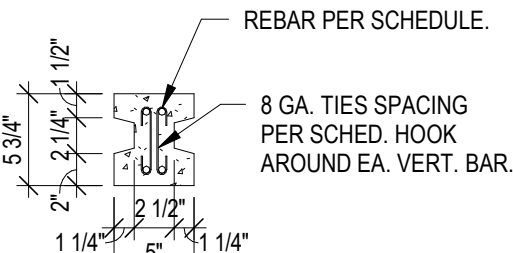
LINE POST
