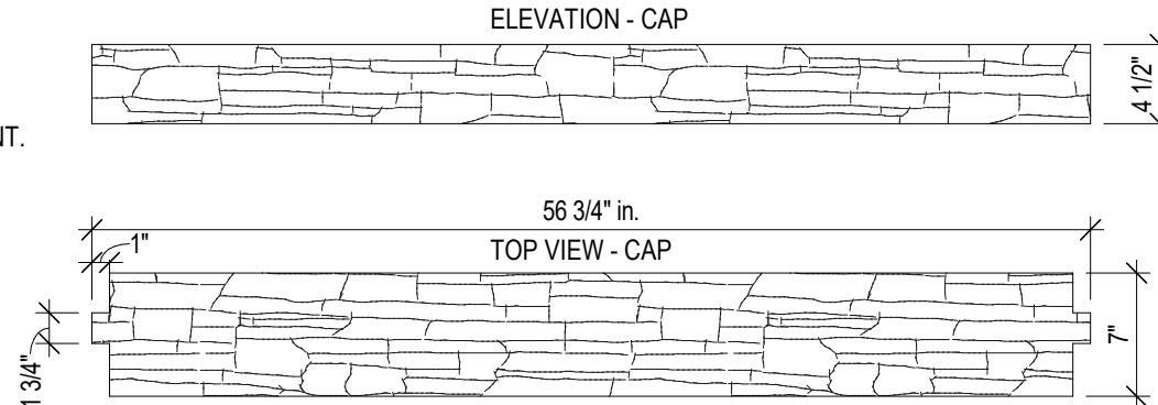
PANEL CAP
