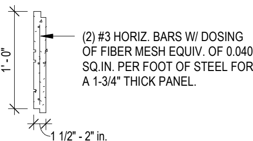
PANEL - SECTION
