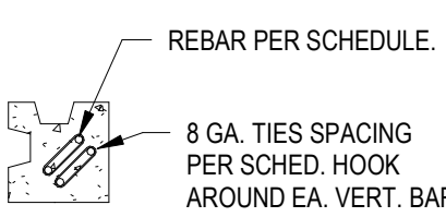
CORNER POST
