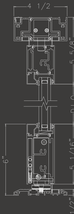
Head and Sill
