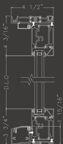
Head and Sill
