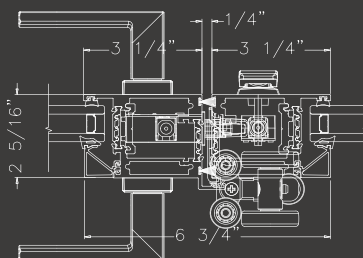
Astragal Left Carrier Set
