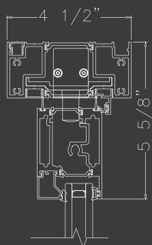
Head with Door Stop
