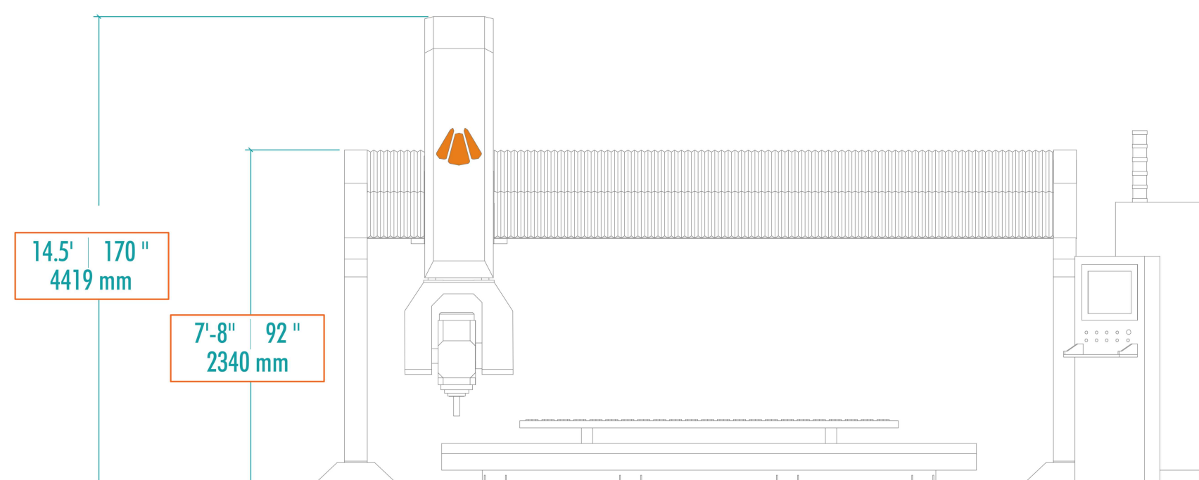
FRONT VIEW
