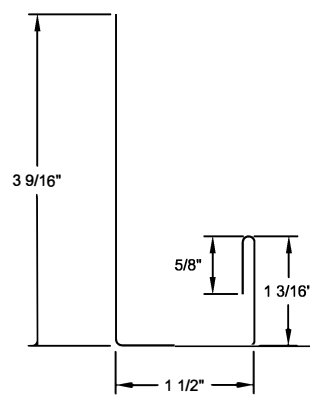
"J" Channel JC-1
