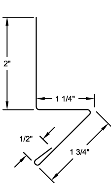
Base Drip BD-2
