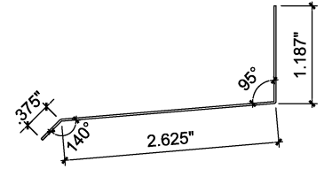
BASE FLASHING DETAIL BF1110 Blank Size 4.062"
