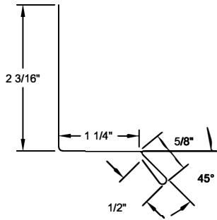
Drip Cap DC-2
