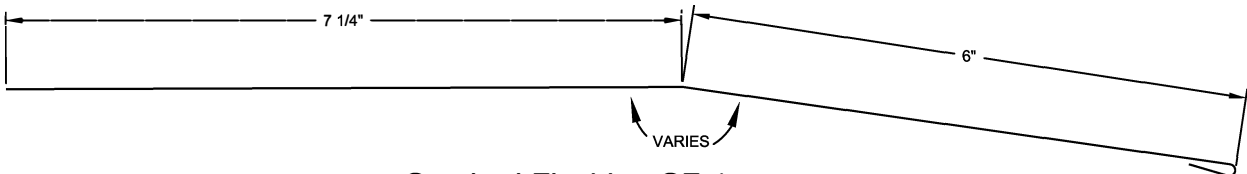
Gambrel Flashing GF-1
