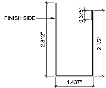
SOFFIT FLASHING DETAIL SF1306 Blank Size 7"
