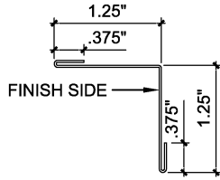
INSIDE CORNER TRIM DETAIL IC1105 Blank Size 3.25"
