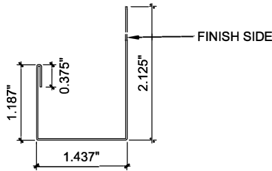
BASE FLASHING DETAIL BF1301 Blank Size 5"
