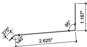
BASE FLASHING DETAIL BF1110 Blank Size 4.062"
