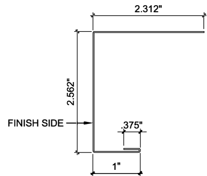
JAMB FLASHING DETAIL JF1109 Blank Size 6.187"
