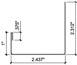
BASE FLASHING DETAIL BF1118 Blank Size 6.062"
