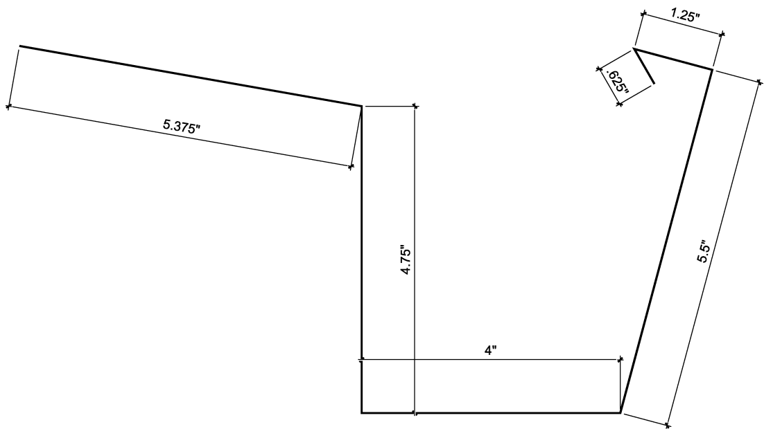
BOX GUTTER PRE-HUNG GU9004 Blank Size 21.5"
