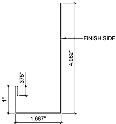
BASE FLASHING DETAIL BF1107 Blank Size 7.062"
