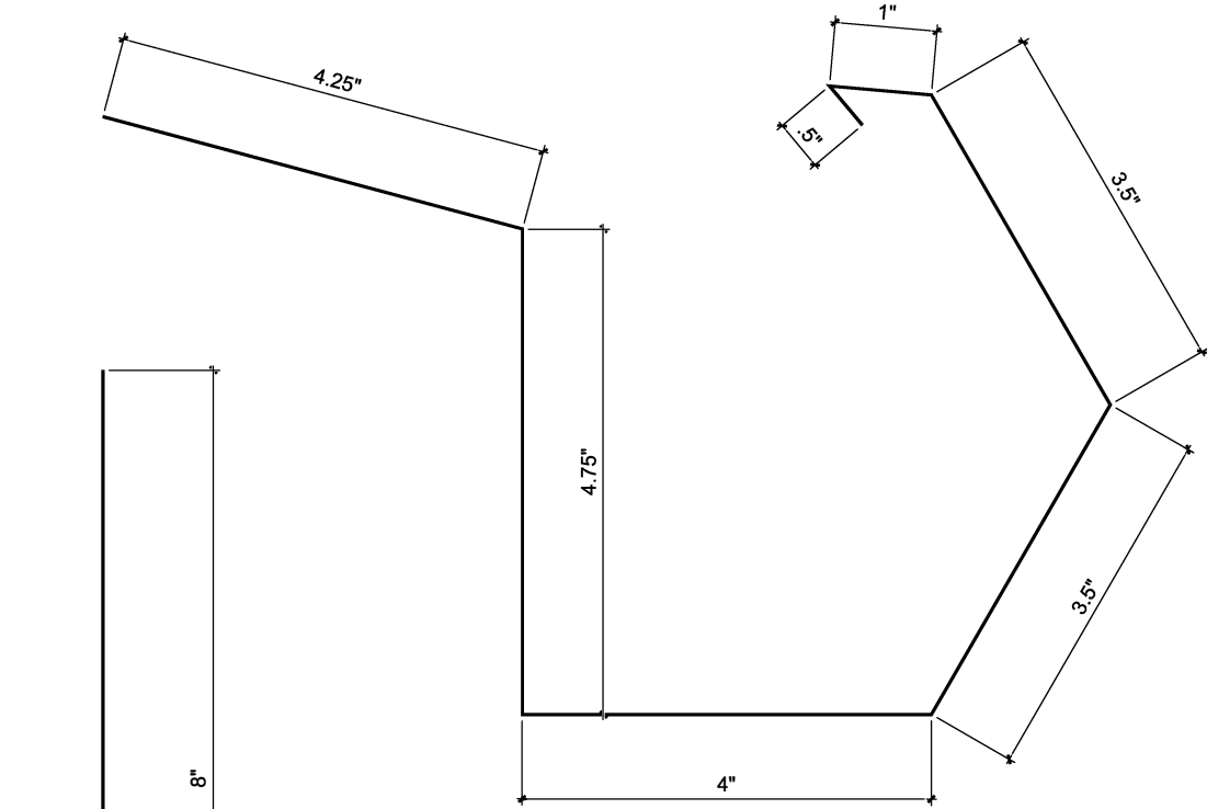
SCULPTURED GUTTER PRE-HUNG GU9006 Blank Size 21.5"
