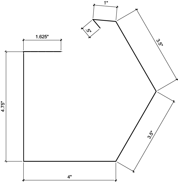
SCULPTURED GUTTER POST-HUNG GU9007 Blank Size 18.875"
