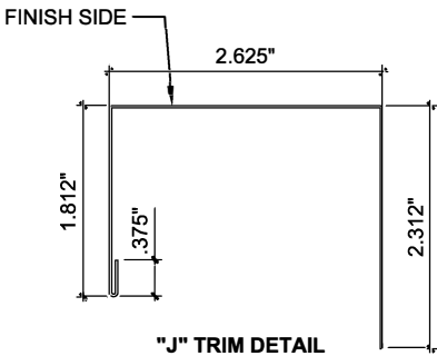
"J" TRIM DETAIL JT1119 Blank Size 7.125"
