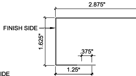
SOFFIT FLASHING DETAIL SF1108 Blank Size 6.062"
