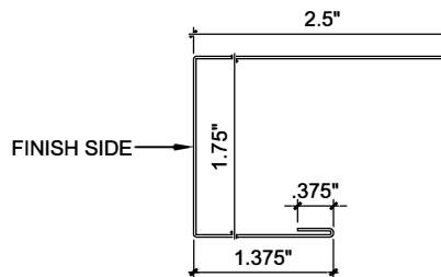
SOFFIT FLASHING DETAIL SF1116 Blank Size 6"
