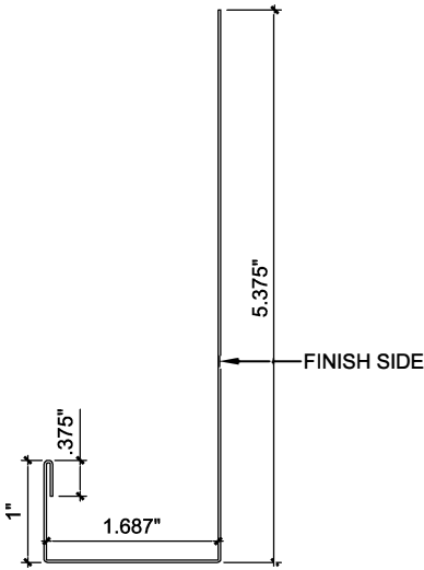
BASE FLASHING DETAIL BF1115 Blank Size 8.437"
