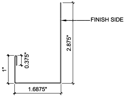
BASE FLASHING DETAIL BF1101 Blank Size 5.875"
