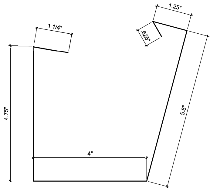
BOX GUTTER POST-HUNG GU9005 Blank Size 17.375"
