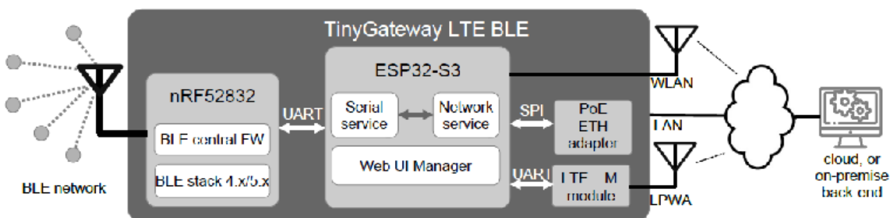
TinyGateway LTE BLE: architecture and interfaces
