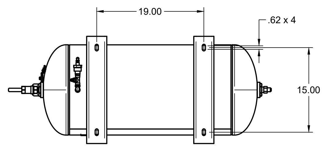
BOTTOM VIEW
