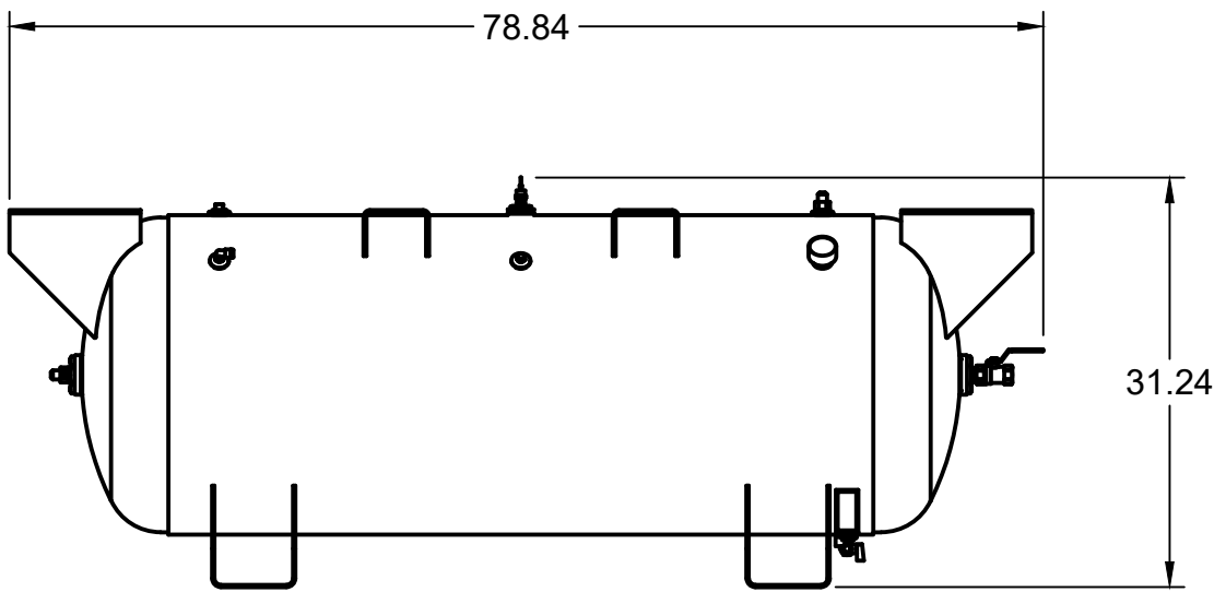
FRONT VIEW
