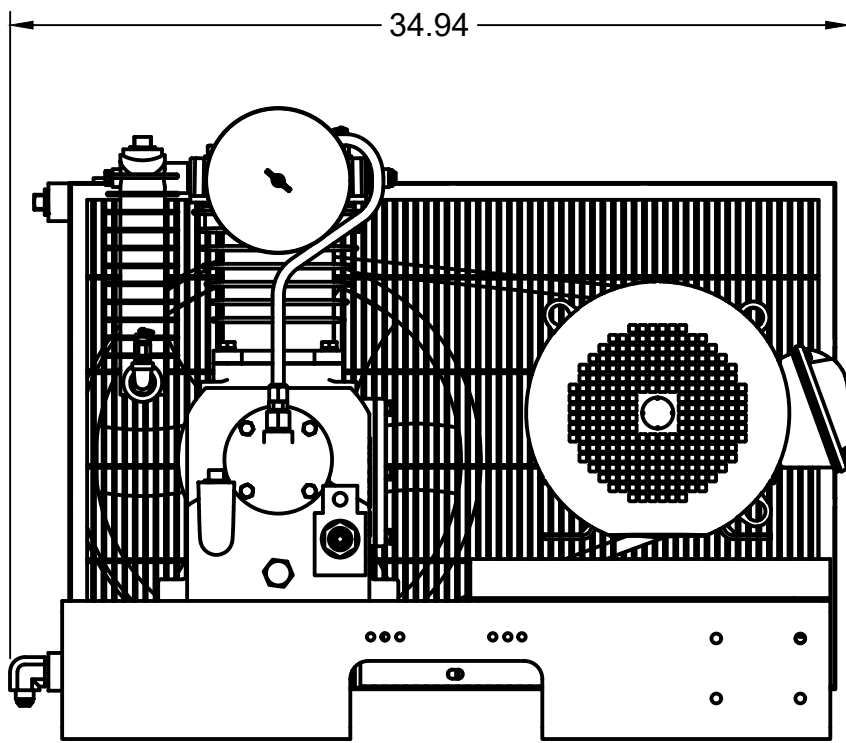
FRONT VIEW
