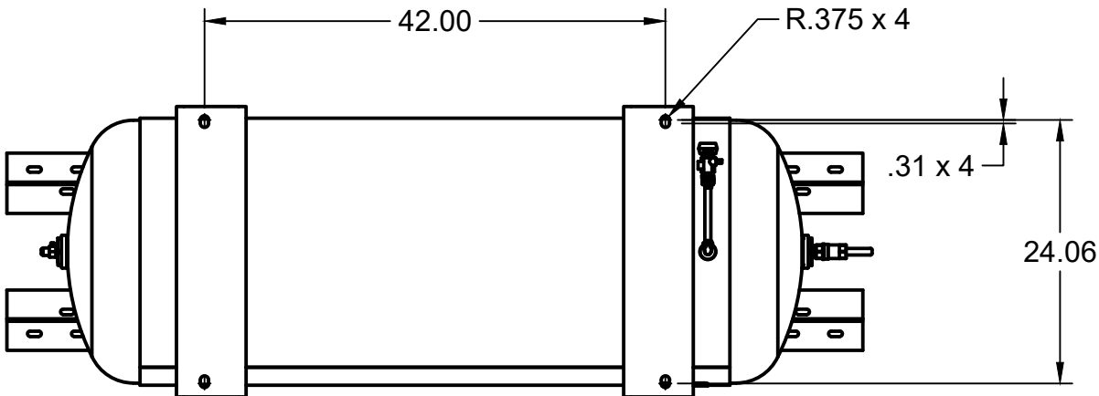
BOTTOM VIEW
