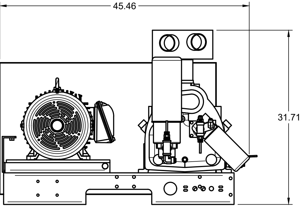
FRONT VIEW
