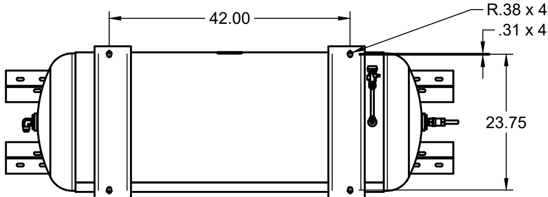
BOTTOM VIEW
