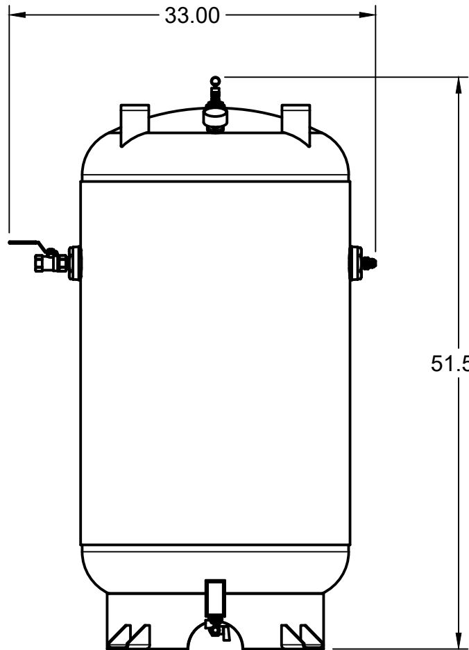
FRONT VIEW
