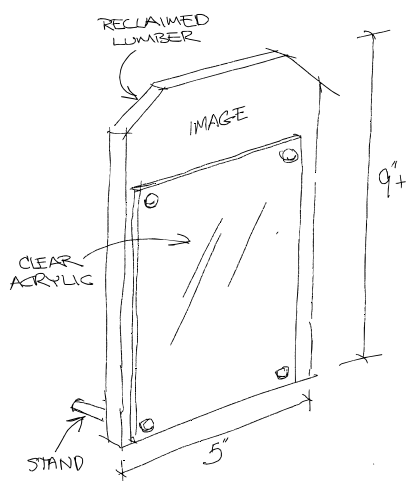
SMALL FRAME - SMF FOR 4 x 6 PHOTO
