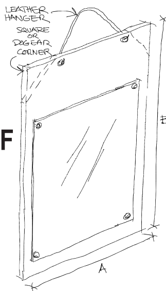
MEDIUM FRAME - MDF FOR 5 x 7 PHOTO (A) 5.5" x (B) 11"
