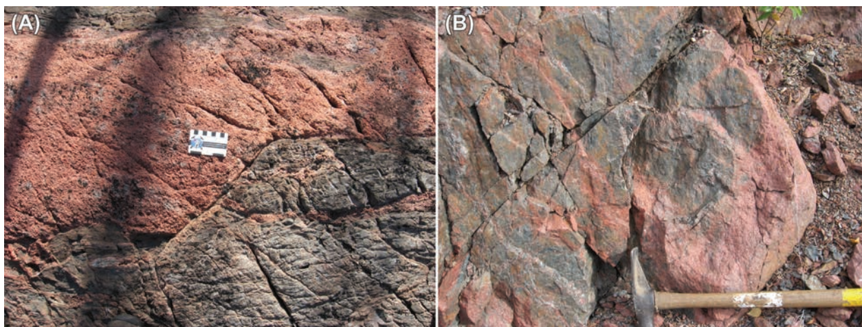
Figure 6. (A) Pink leucogranite dike with disseminated and fracture-hosted U-mineralization intruding orthogneiss and (B) texturally similar alteration (episyenite) propagating along fractures in gneiss at the Dubyna pit. NRCan photos 2021-232 and 2021-233.
