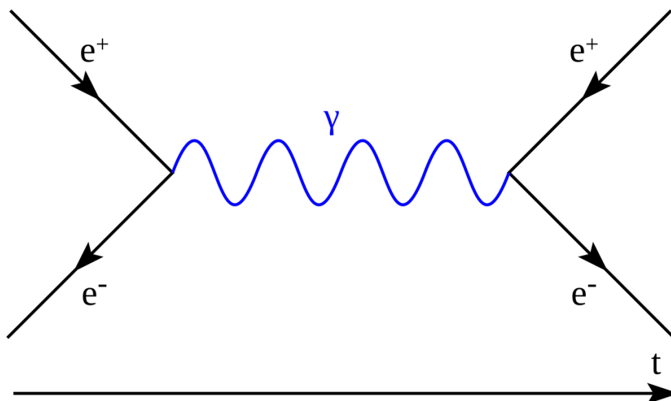
A Feynman diagram showing the annihilation of an electron and a positron (antielectron), creating a photon that later decays into a new electron–positron pair.
