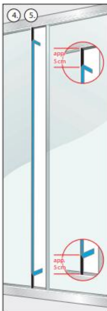
4. Remove approximately 5cm of the Liner at the bottom and the top and turn it to the back side. 5. Slide the glasses together and adjust vertical fitting of both glass walls.
