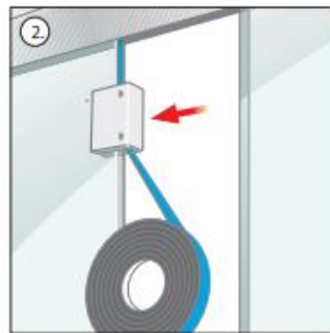
2. Apply the tape to one edge of the glass. By using the tesa® edge applicator a straight line and quick assembly will be assured.
