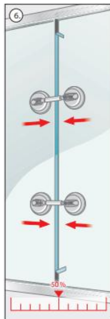
6. Join the glass panels together by using medium force of the vacuum device before removing the liner.
