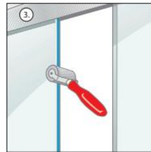
3. Pressure is essential for good adhesion performance and to avoid air bubbles. For optimal results we recommend a uniform pressure during application e.g. by a pressure roller.
