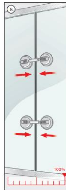
8. Final adjustment of force to reach optimal bonding results of both glass edges.
