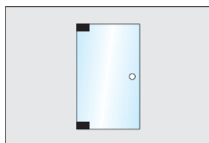
top patch fitting bottom patch fitting max. 1.200 x 2.800 mm max. 120 kg
