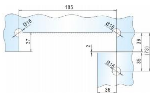
Transom/sidepanel pivot patch fitting Transom/sidepanel connector
