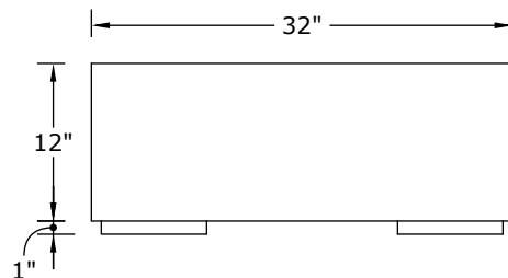
SIDE ELEVATION
