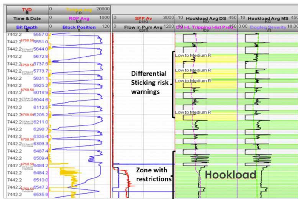
Figure 7—Example annotated screenshot taken from a live operation in South America where the operator's monitoring engineers observed stuck pipe risk warnings (Differential Sticking) while tripping prior to a risk zone, and advised corrective actions to the rig. After following recommendations to ream and move through with pipe rotation, the risk zone was passed without incident. Data is visualized in a 3rd party commercial WITSML viewer.
