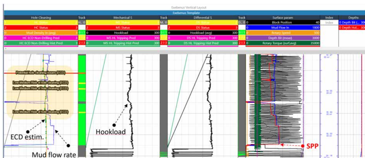
Figure 8—Example case from a live field test on a conventional offshore well, where Hole Cleaning risk warnings were raised (leftmost track, in shaded area) The vertical position of the alert text corresponds to the notification time. Curves for estimated ECD, mud flow rate, standpipe pressure and hookload have been annotated. The drilling data is visualized in a third party commercial WITSML viewer. Upon notifying the rig site, the shakers were checked and excessive cuttings were observed in the returns, which prompted remedial actions to be taken.
