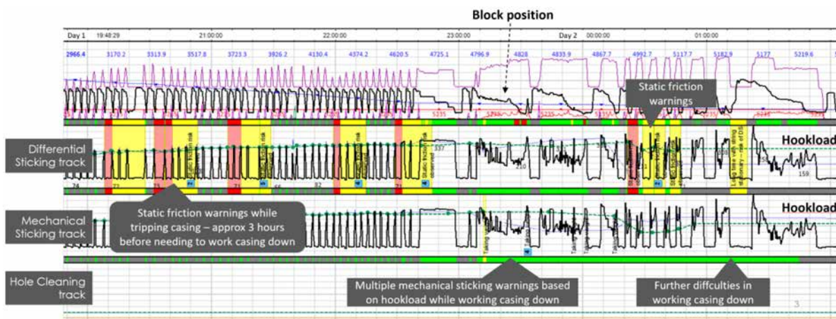
Figure 4—Example test scenario from historical data with static friction warnings (differential sticking risk) and mechanical restriction symptoms visible in the hookload measurements while running in casing prior to a period with restrictions. Historical surface data from the operation and the stuck pipe risk outputs are visualized in a commercial WITSML viewer.
