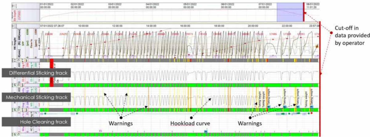
Figure 5—A blind test data interval visualized using a commercial WITSML viewer. Mechanical sticking warnings are raised with increasing frequency and severity over the displayed interval. Orange warnings indicate a higher risk severity than yellow warnings. After the cut-off in the data at the end of the interval, a stuck pipe incident occurred.
