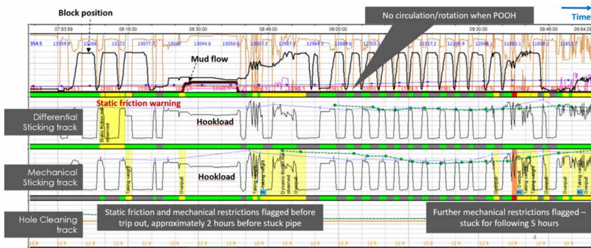
Figure 3—Example test scenario from historical data with mechanical restrictions visible in the hookload measurements while tripping. Historical surface data from the operation and the stuck pipe risk outputs are visualized in a commercial WITSML viewer. Several warnings were raised by the software in advance of the stuck pipe event occurring at the end of this interval.
