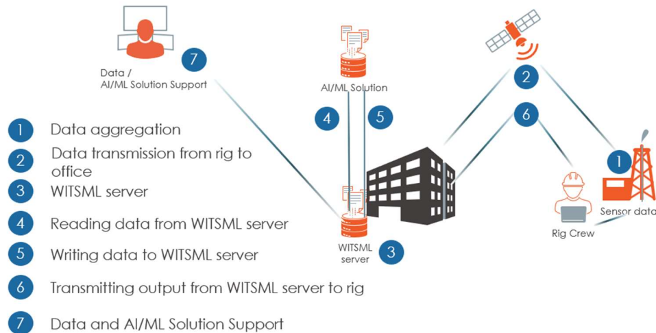
Fig. 1—Typical technical set up of the services: Data Transfers between Wellsite, Office, WITSML Providers, and Drilling Mud Logging Providers
