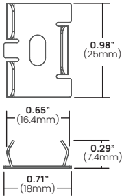
Metal Mounting Clip
