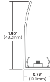
Metal Glare Shield
