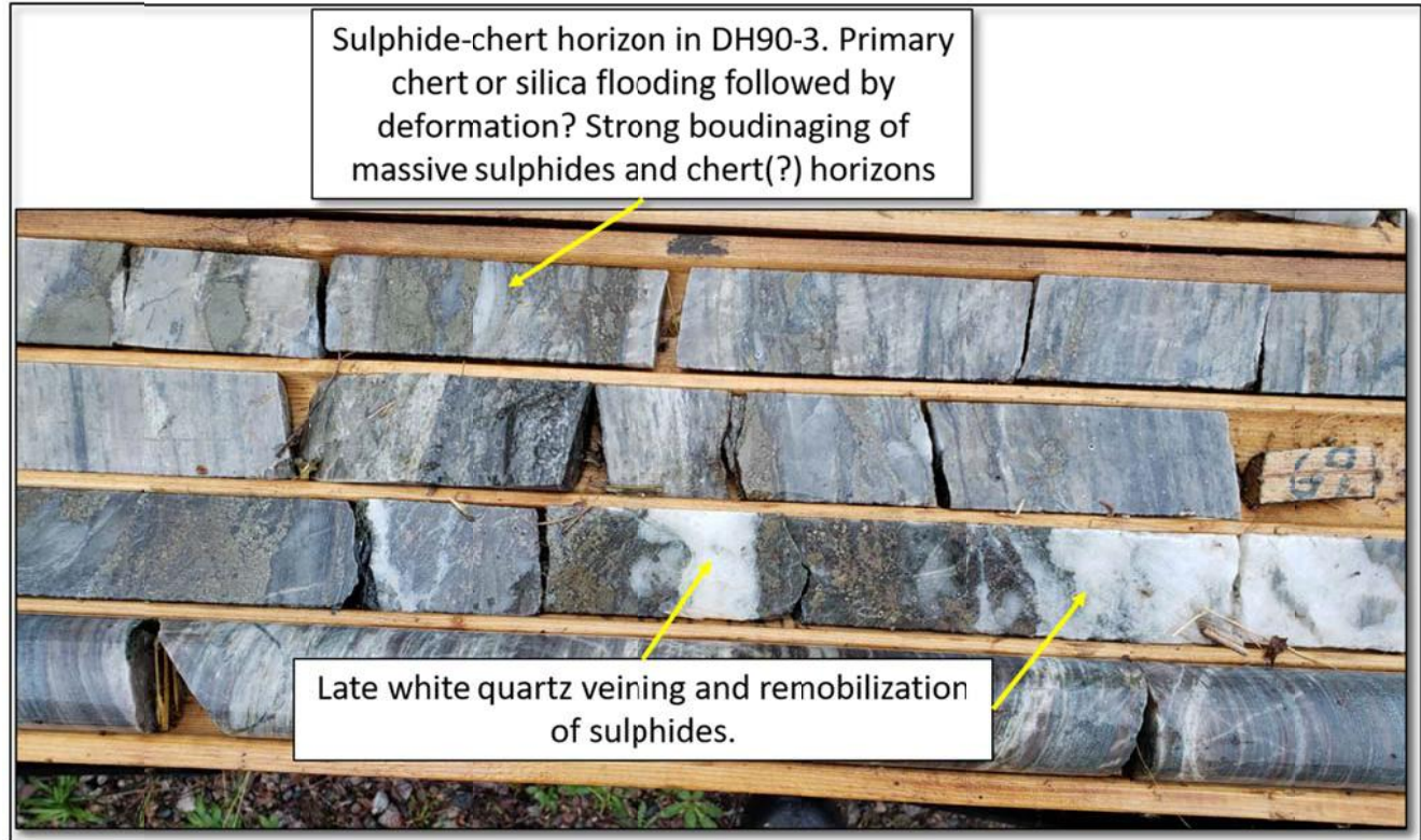
Figure 7.5 Core photograph of drill hole DH90-3 sulphide-chert horizon.
