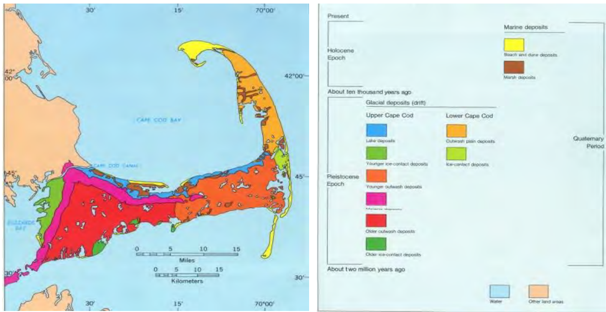
Figure I-2. Geologic map of Cape Cod (generalized from detailed mapping by K. F. Mather, R. P. Goldthwait, L. R. Theismeyer, J. H. Hartshorn, Carl Kotteff, and R. N. Oldale).
