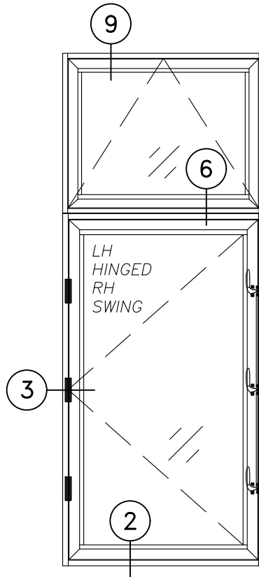
P.O./CAS WINDOW
