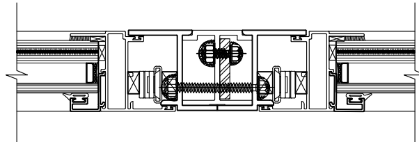
ZERO MULL
