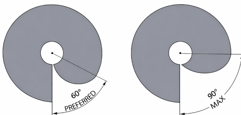
Figure 4: Alternative Helical Plates for Rocky Soils
