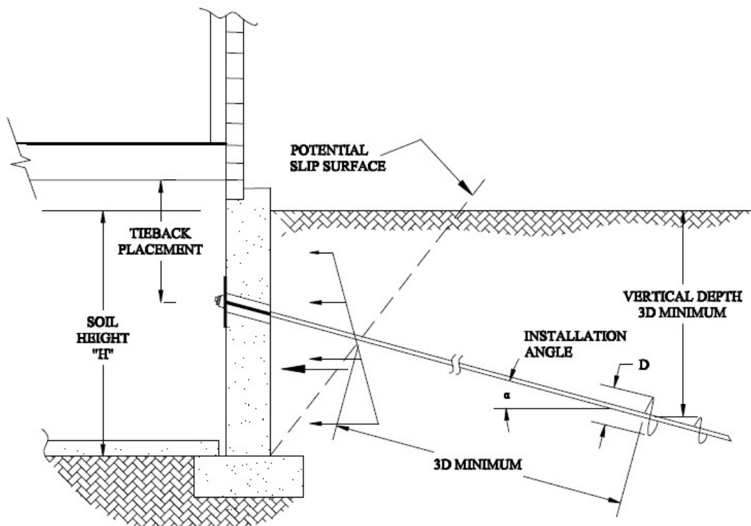
Figure 5: Tieback Application
