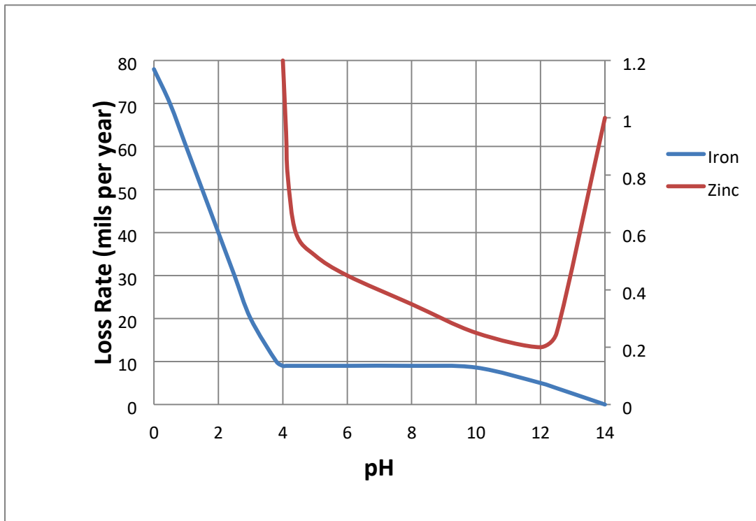
Figure 9: Effect of pH on Corrosion of Iron and Zinc
