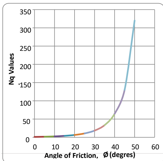
Figure 3: Bearing Capacity Factor, N_q
