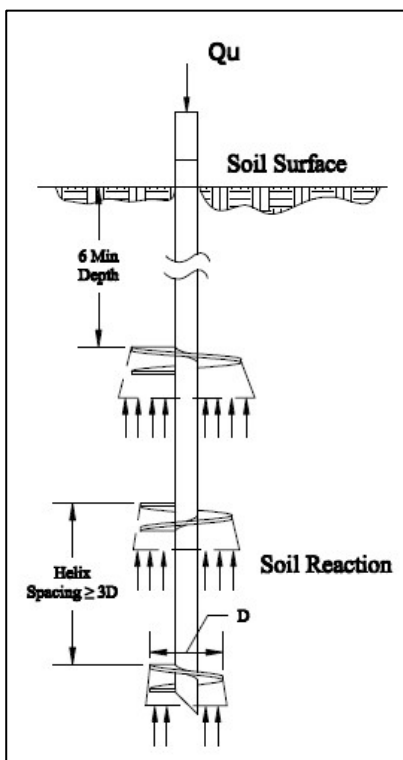
Figure 2: Bearing Capacity Resistance Diagram
