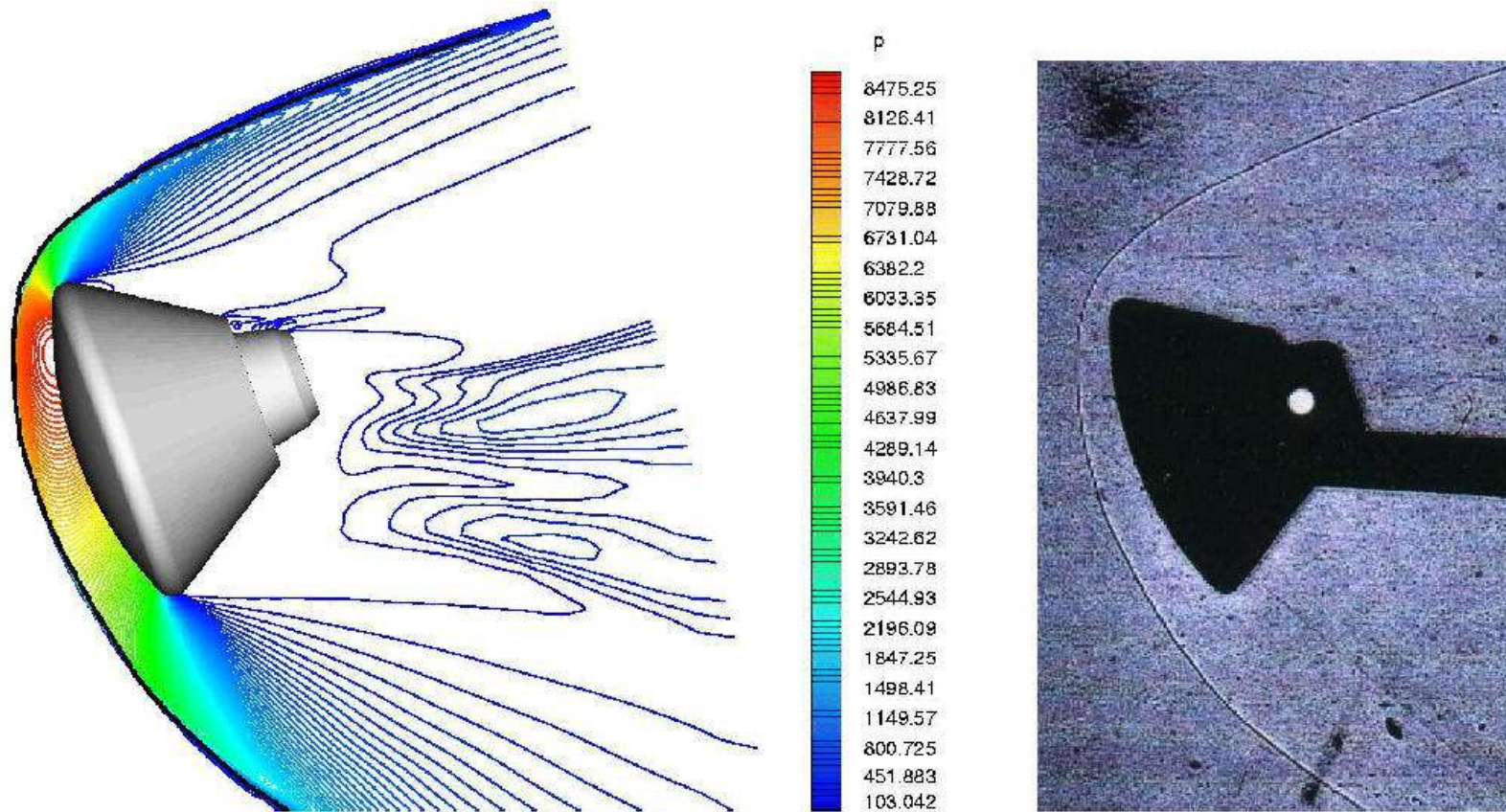
(a) Pressure contour lines. The shock location of the schlieren picture is included.
