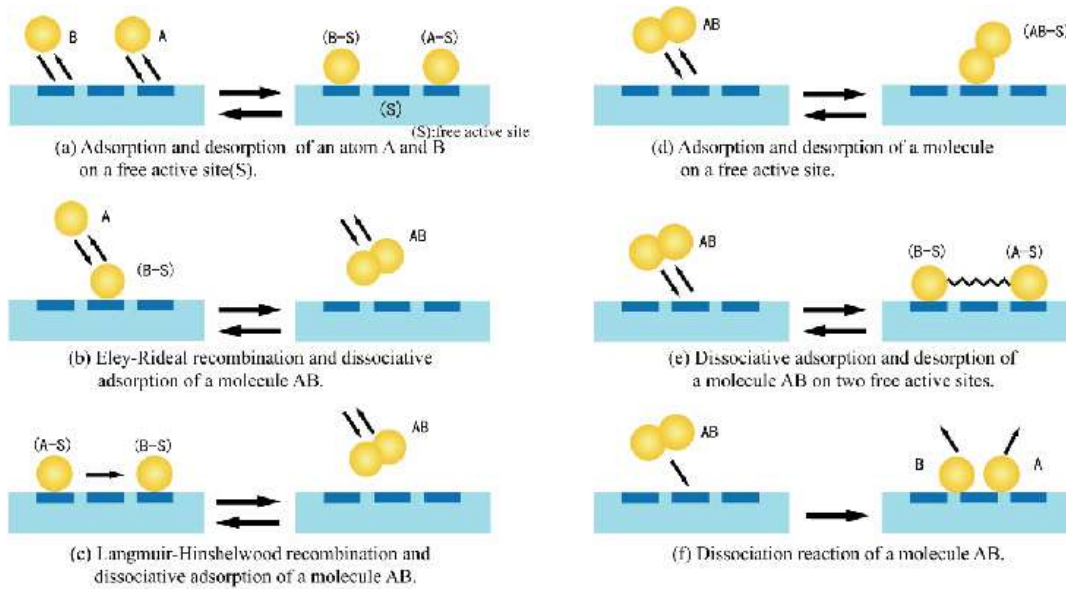
Figure 12 Chemical Processes in Heterogenous Catalysis on Surface
