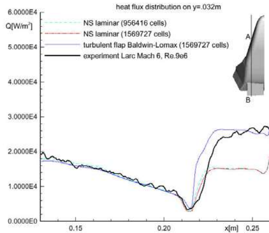
Figure 7 X-38 flap heating at Mach 6.
