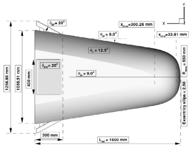
Figure 17 KHEOPS revision 4.2; Side view.
