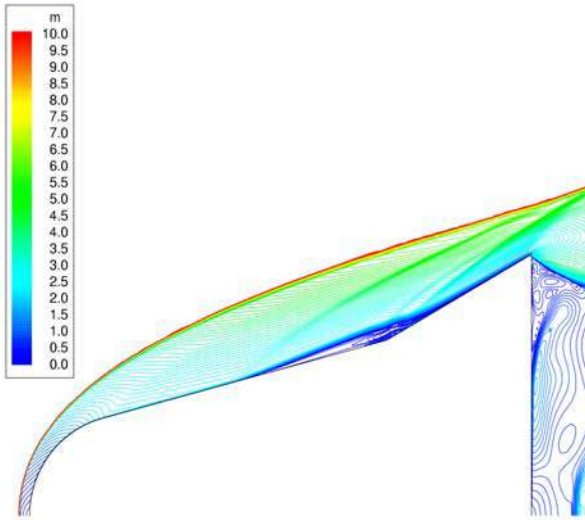
Figure 36 M_\infty = 10 contour plots of axisymmetric NS non-equilibrium computations.
