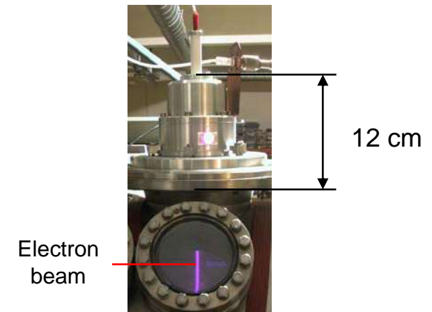
Miniaturised electron gun prototype
