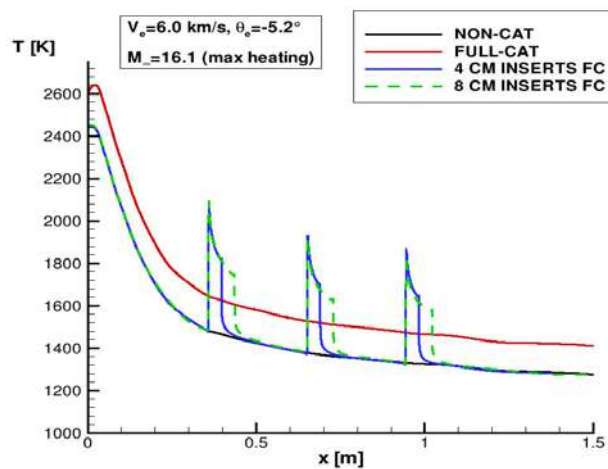
Figure 29 Full Catalytic patches simulation.
