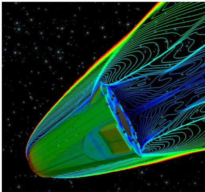
Figure 35 3D Flowfield around the vehicle.
