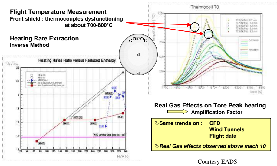
Figure 5 Post-flight analysis of real gas effects on ARD.
