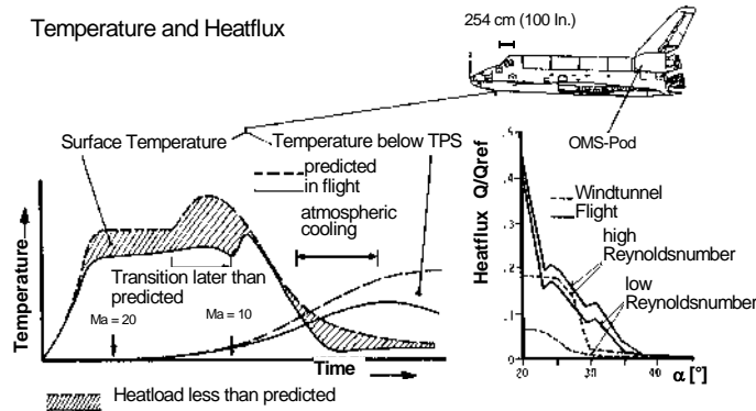
Figure 3 Shuttle heat flux overdimensioning.
