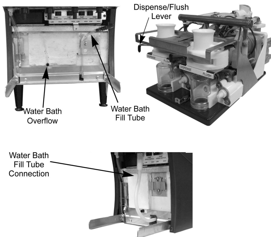
Figure 6. Water Bath and Dispense/Flush Lever
