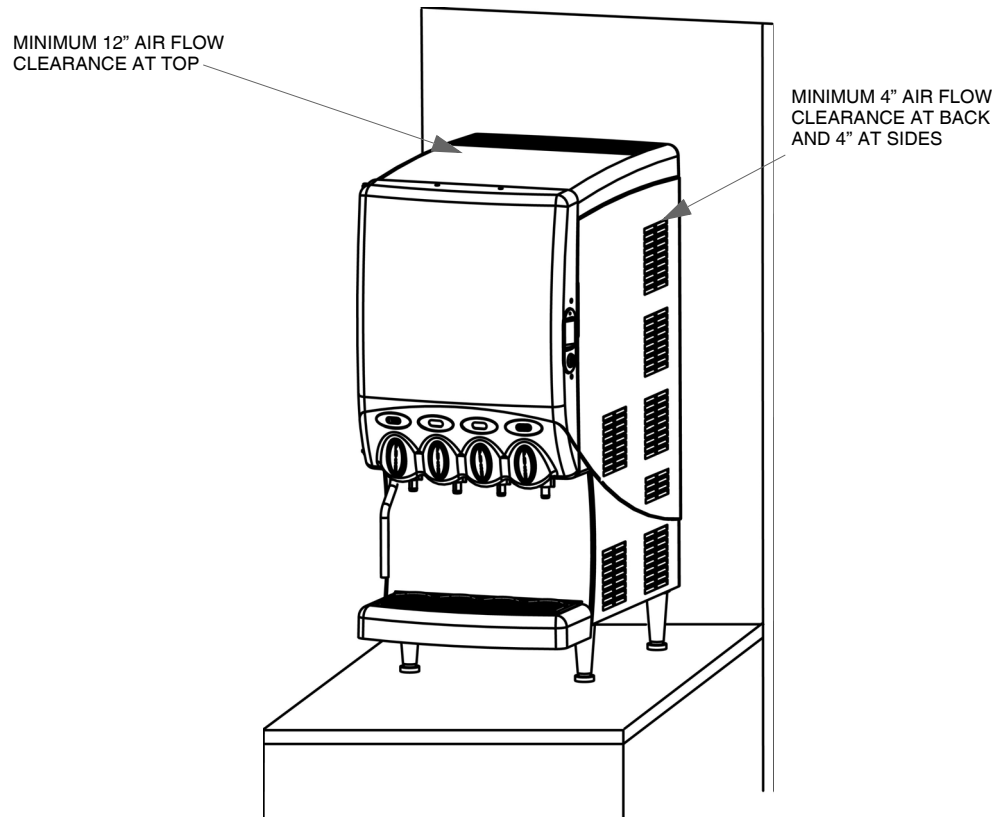
Figure 5. Minimum Clearances
