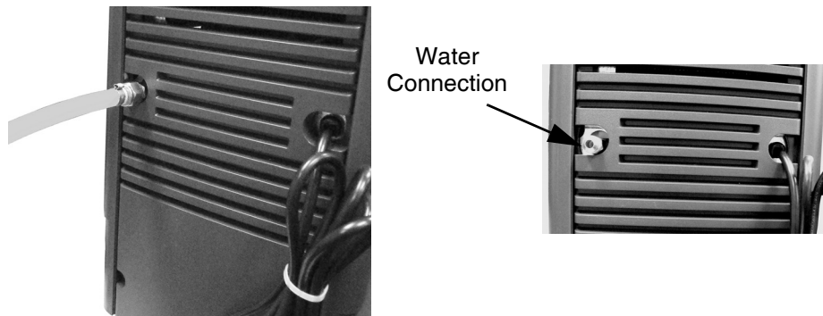
Figure 4. Plumbing Connection
