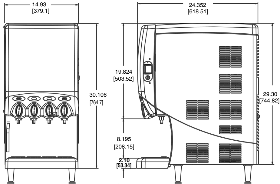
Figure 1. Unit Dimensions
