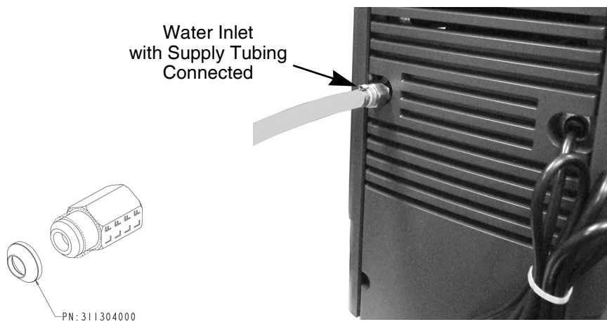
Figure 8. Water Supply Connection on Rear of Unit
