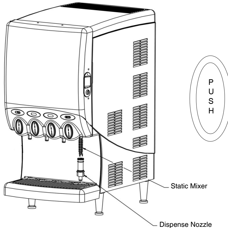
Figure 9. Dispense Nozzle
