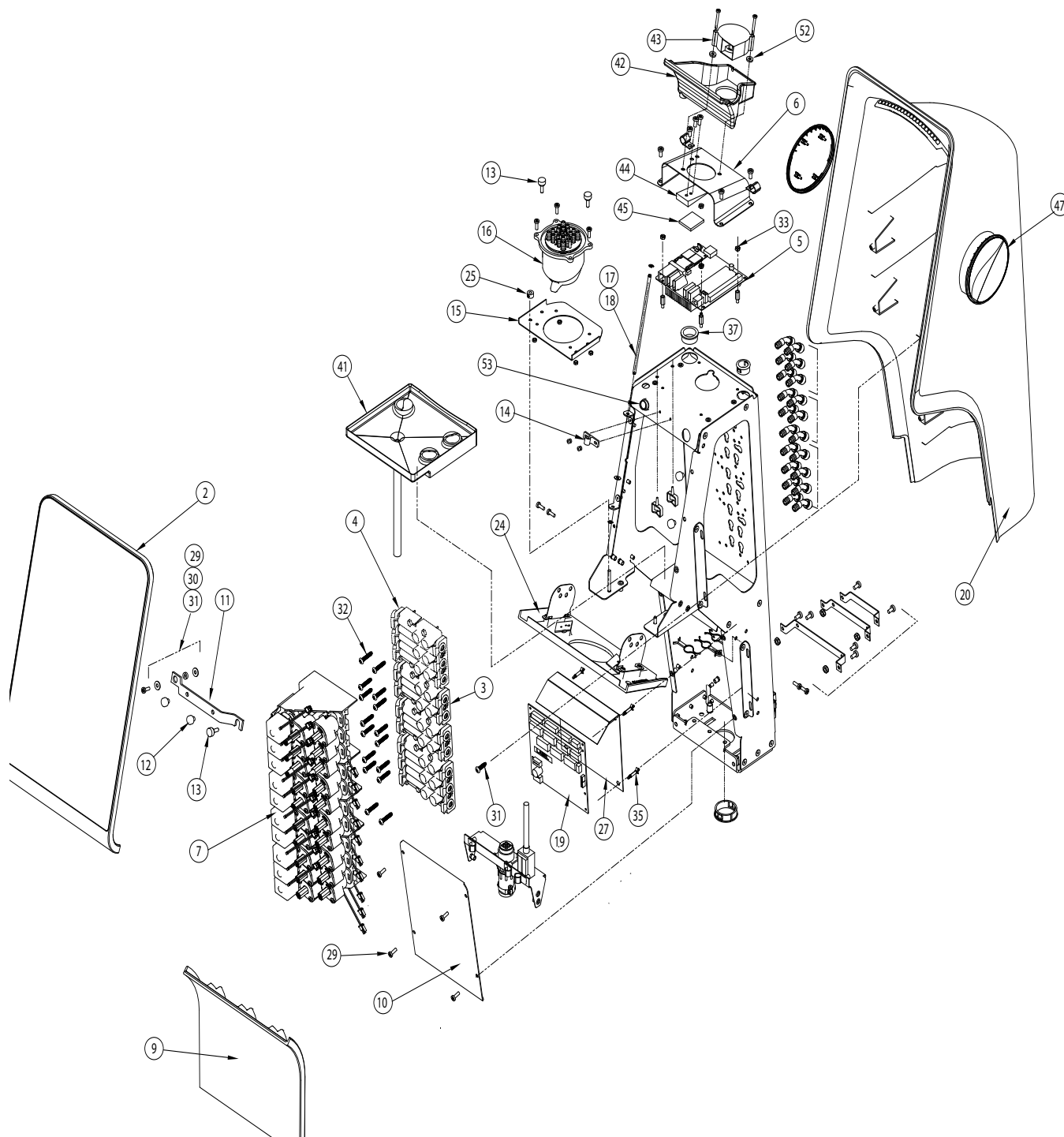
Figure 1. Tower Assembly
