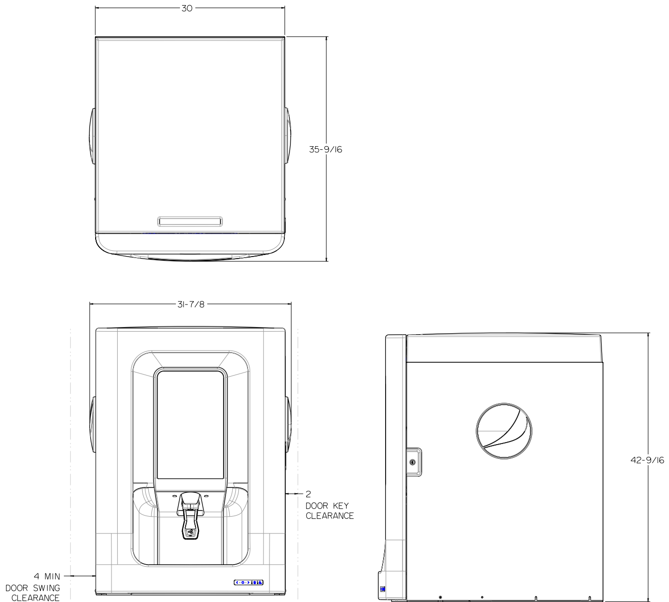
Figure 1. Spire 4.1 Physical Dimensions
