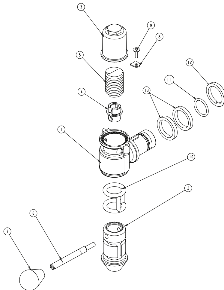
Figure 4. Assemblé Valve Marchandiseur
