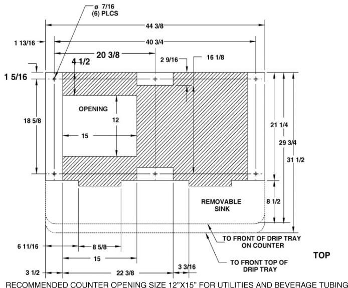
Figure 4.Mounting Template
