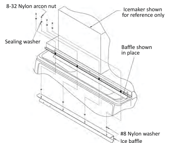
Figure 5.Baffle Kit
