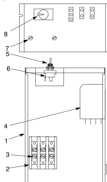
FIGURE 3. ELECTRICAL BOX ASSEMBLY
