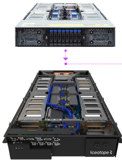
100% LIQUID-COOLED
