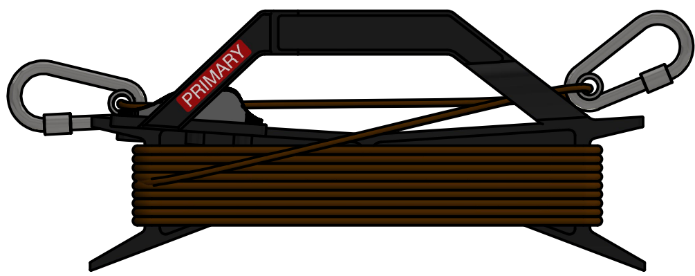
QTY: (4) 350G HEAVY GUY ROPE W/CLEAT-14M-PRIMARY P/N: 350G-P-GC14-PRI-RED 1.5 lbs / 0.7 kg (each)
