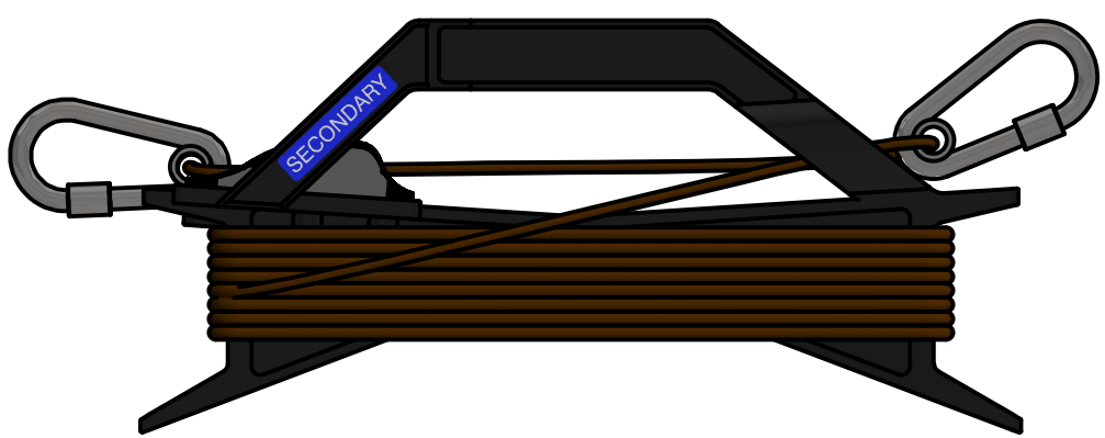
QTY: (4) 350G HEAVY GUY ROPE W/CLEAT-14M-SECONDARY P/N: 350G-P-GC14-2ND-BLU 1.4 lbs / 0.6 kg (each)
