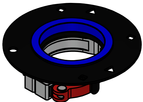
QTY: (1) SECONDARY GUY RING-350 P/N: BSM3-A-M100-RNG-CL0 1.5 lbs / 0.7 kg
